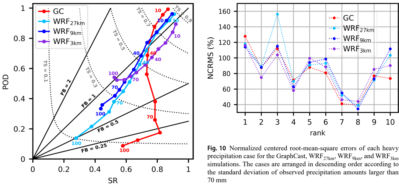
Fig. 9 Performance diagram by different precipitation thresholds for the GraphCast, WRF 27km , WRF 9km , and WRF 3km simulations
